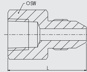
Female-male connection adapter Nominal pressure: 15,000 psi [1,034 bar]
